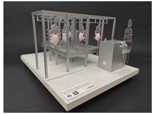
Model of chicken washing system
