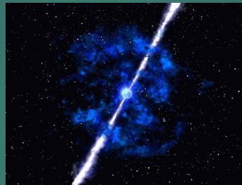
(c) NASA Imaginary picture of gamma-ray burst
